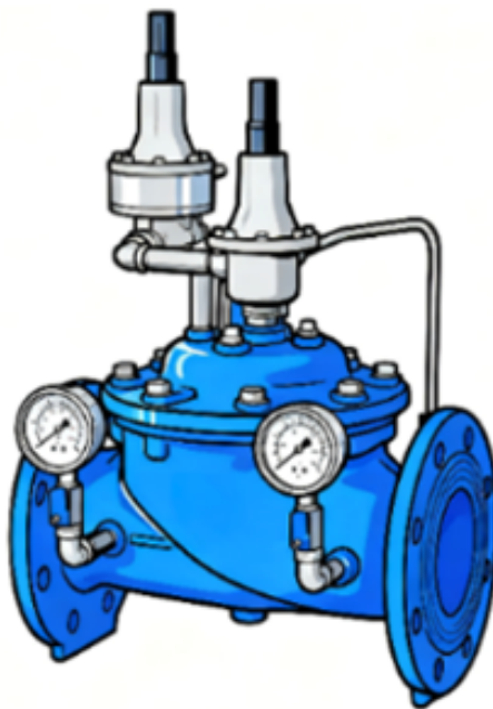
Pressure Reducing and Relief Valve (/portal/article/index/id/172.html)
